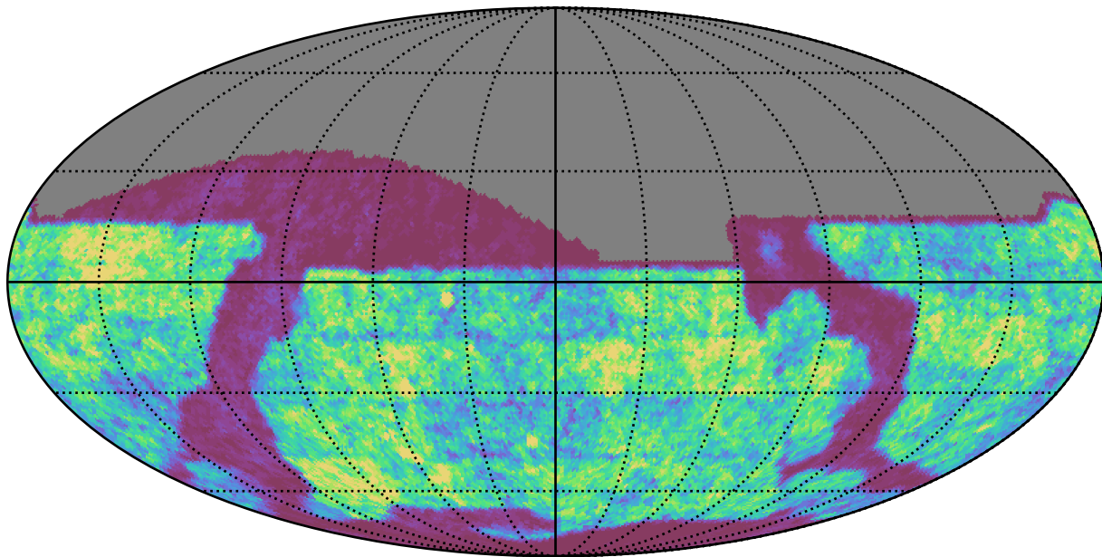
smc_lmc_v3.3_10yrs z band: Gaps_24hr
