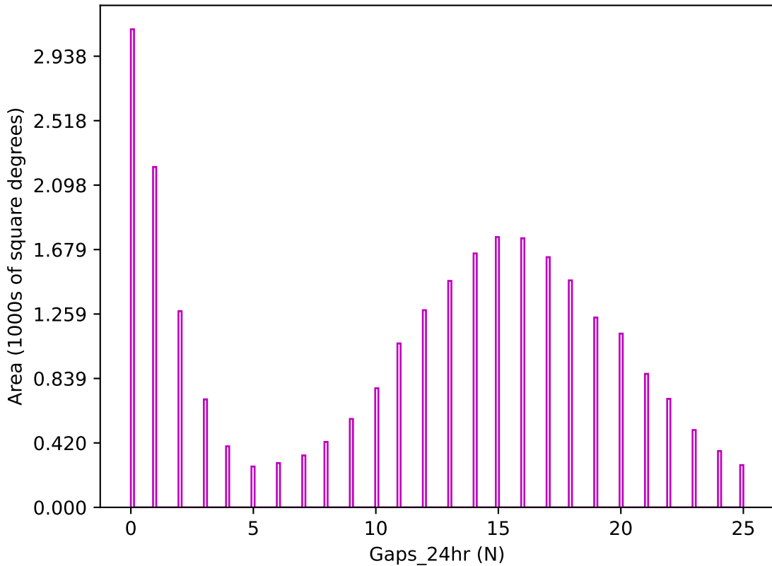
smc_lmc_v3.3_10yrs z band: Gaps_24hr
