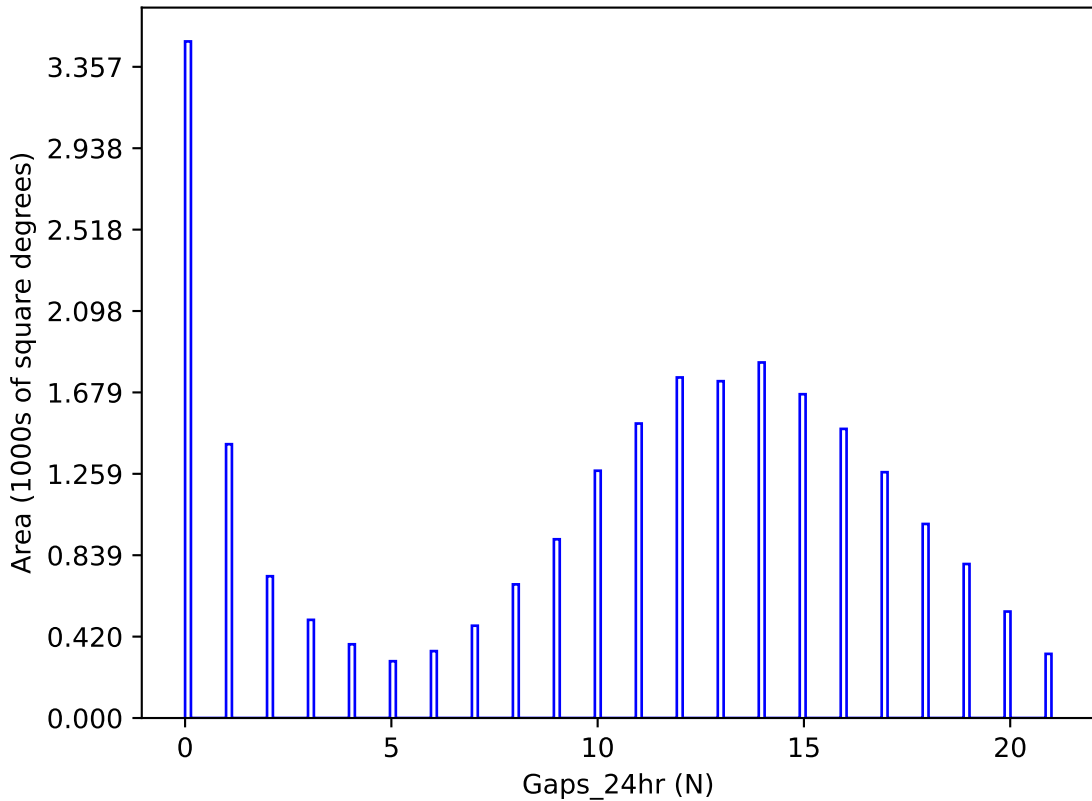
smc_lmc_v3.3_10yrs y band: Gaps_24hr
