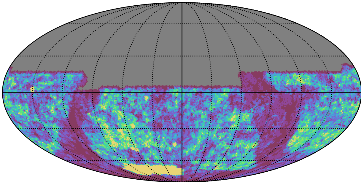
smc_lmc_v3.3_10yrs u band: Gaps_24hr
