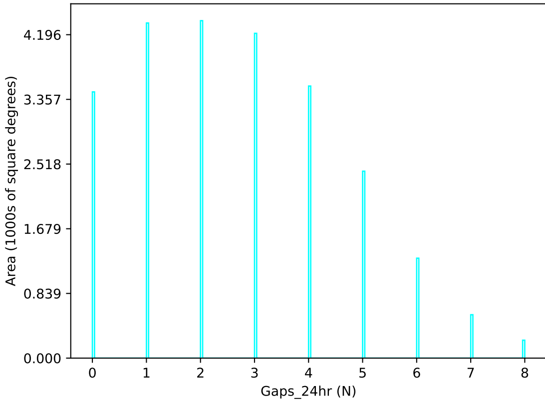
smc_lmc_v3.3_10yrs u band: Gaps_24hr
