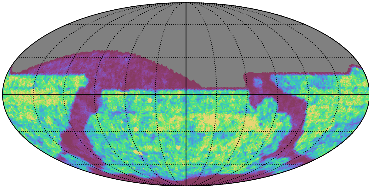
smc_lmc_v3.3_10yrs i band: Gaps_24hr
