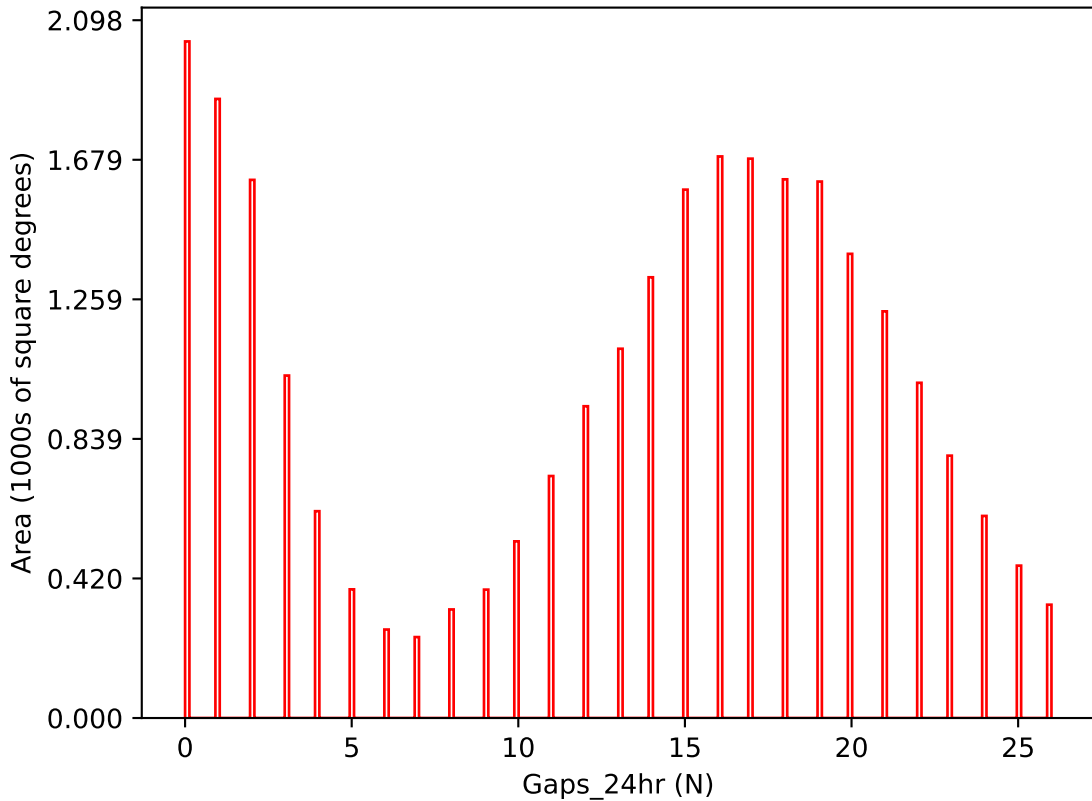
smc_lmc_v3.3_10yrs i band: Gaps_24hr
