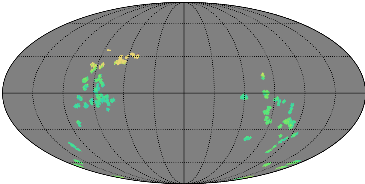
smc_lmc_v3.3_10yrs : GalplaneTimePerFilter_zucker_sfr_map_z
