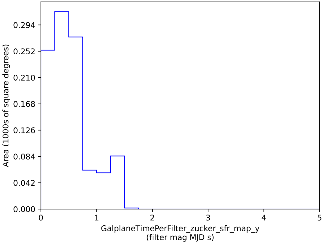
smc_lmc_v3.3_10yrs : GalplaneTimePerFilter_zucker_sfr_map_y
