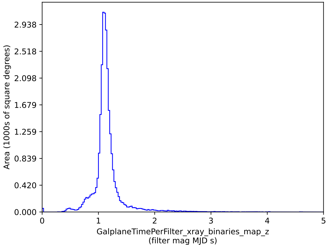
smc_lmc_v3.3_10yrs : GalplaneTimePerFilter_xray_binaries_map_z
