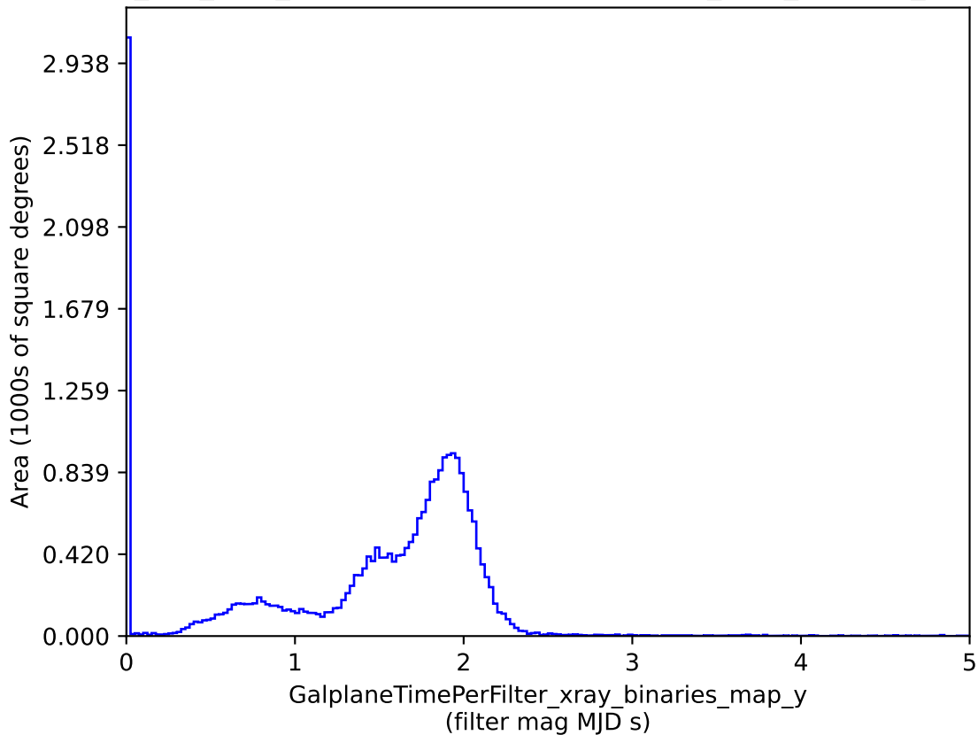
smc_lmc_v3.3_10yrs : GalplaneTimePerFilter_xray_binaries_map_y
