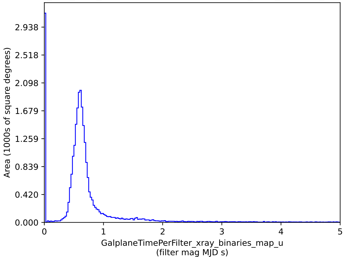
smc_lmc_v3.3_10yrs : GalplaneTimePerFilter_xray_binaries_map_u
