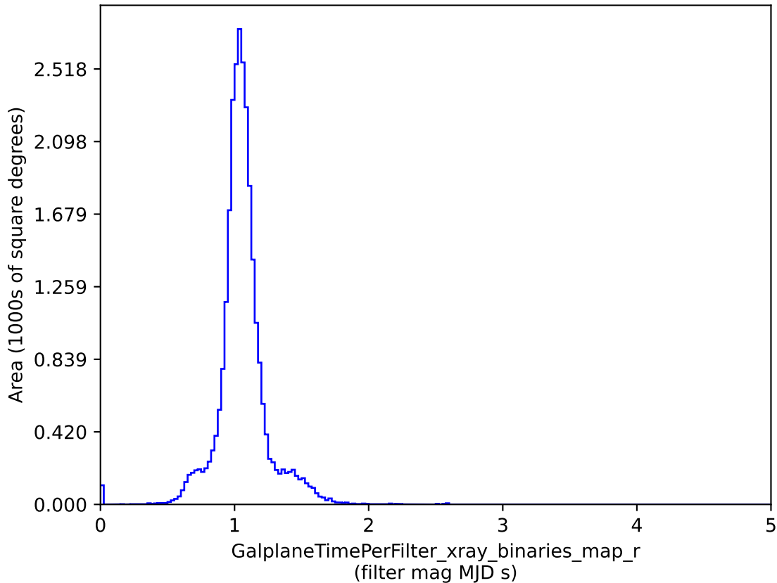
smc_Imc_v3.3_10yrs : GalplaneTimePerFilter_xray_binaries_map_r
