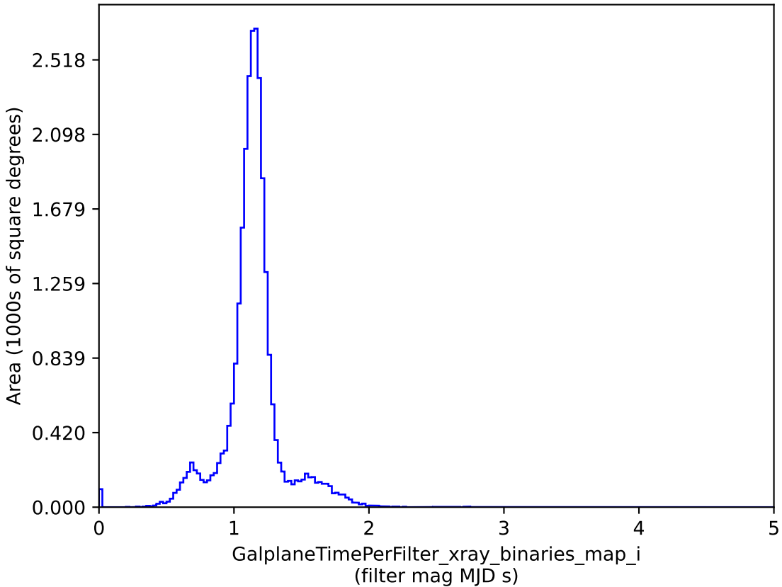
smc_lmc_v3.3_10yrs : GalplaneTimePerFilter_xray_binaries_map_i
