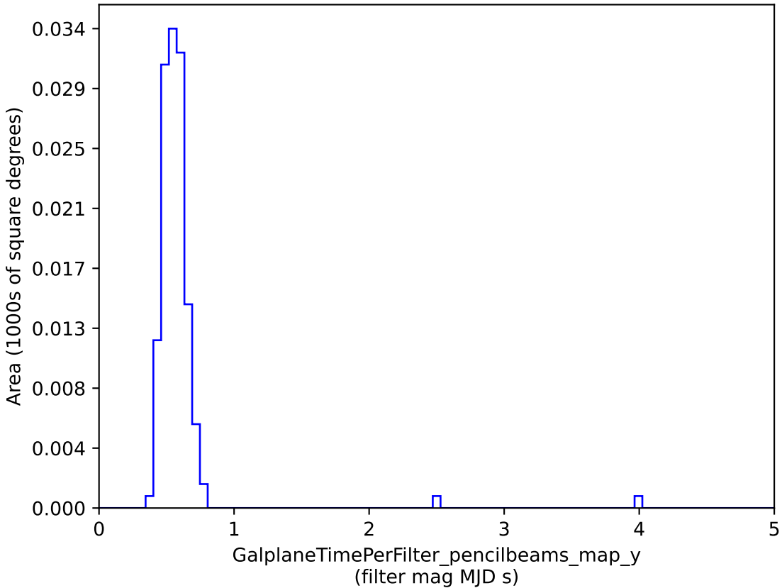
smc_lmc_v3.3_10yrs : GalplaneTimePerFilter_pencilbeams_map_y
