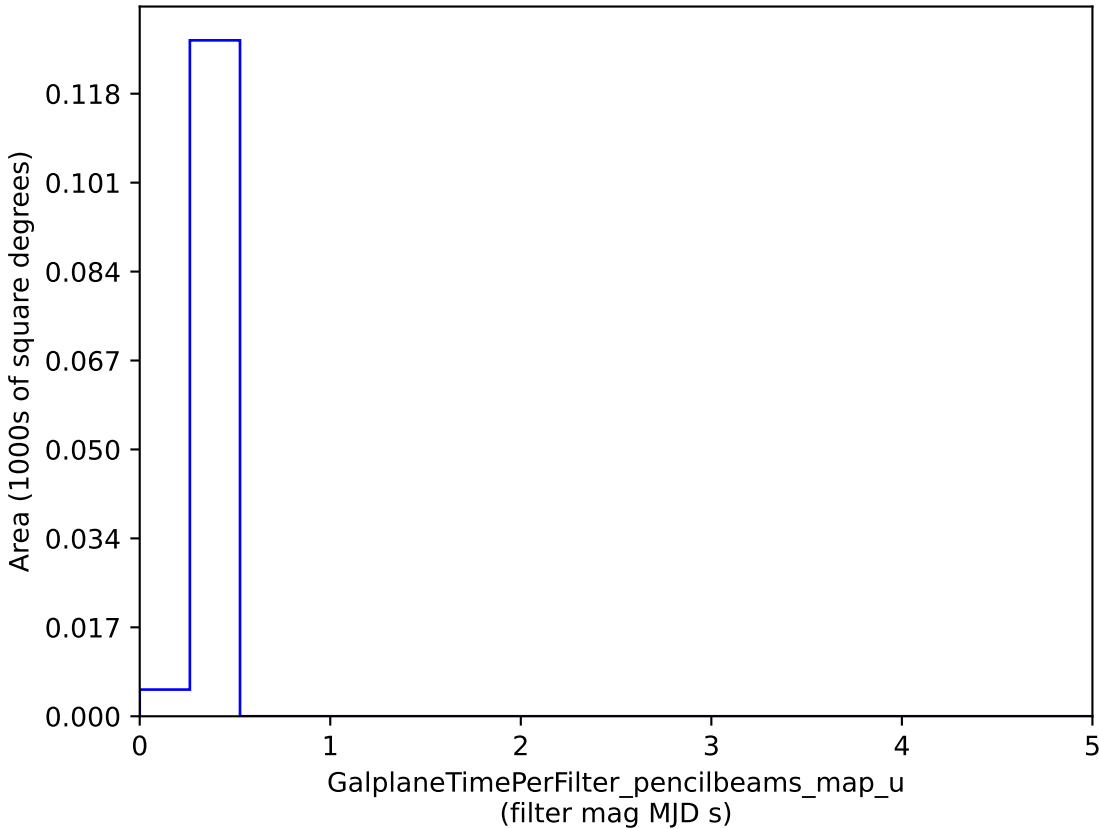
smc_lmc_v3.3_10yrs : GalplaneTimePerFilter_pencilbeams_map_u
