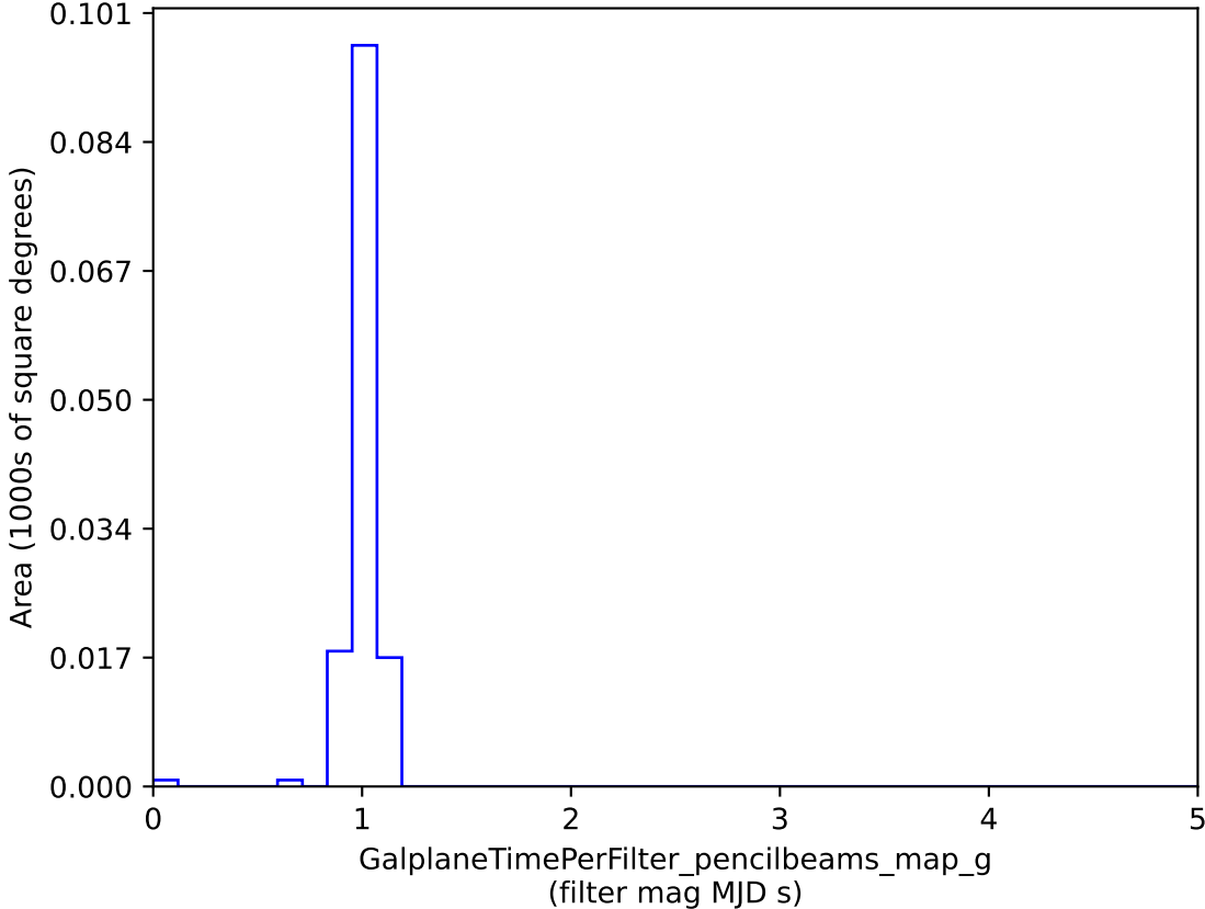
smc_lmc_v3.3_10yrs : GalplaneTimePerFilter_pencilbeams_map_g
