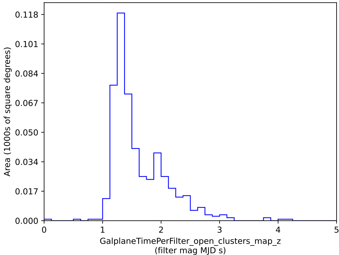
smc_lmc_v3.3_10yrs : GalplaneTimePerFilter_open_clusters_map_z
