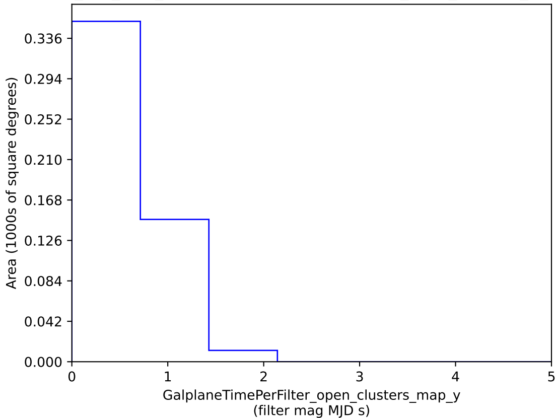
smc_lmc_v3.3_10yrs : GalplaneTimePerFilter_open_clusters_map_y
