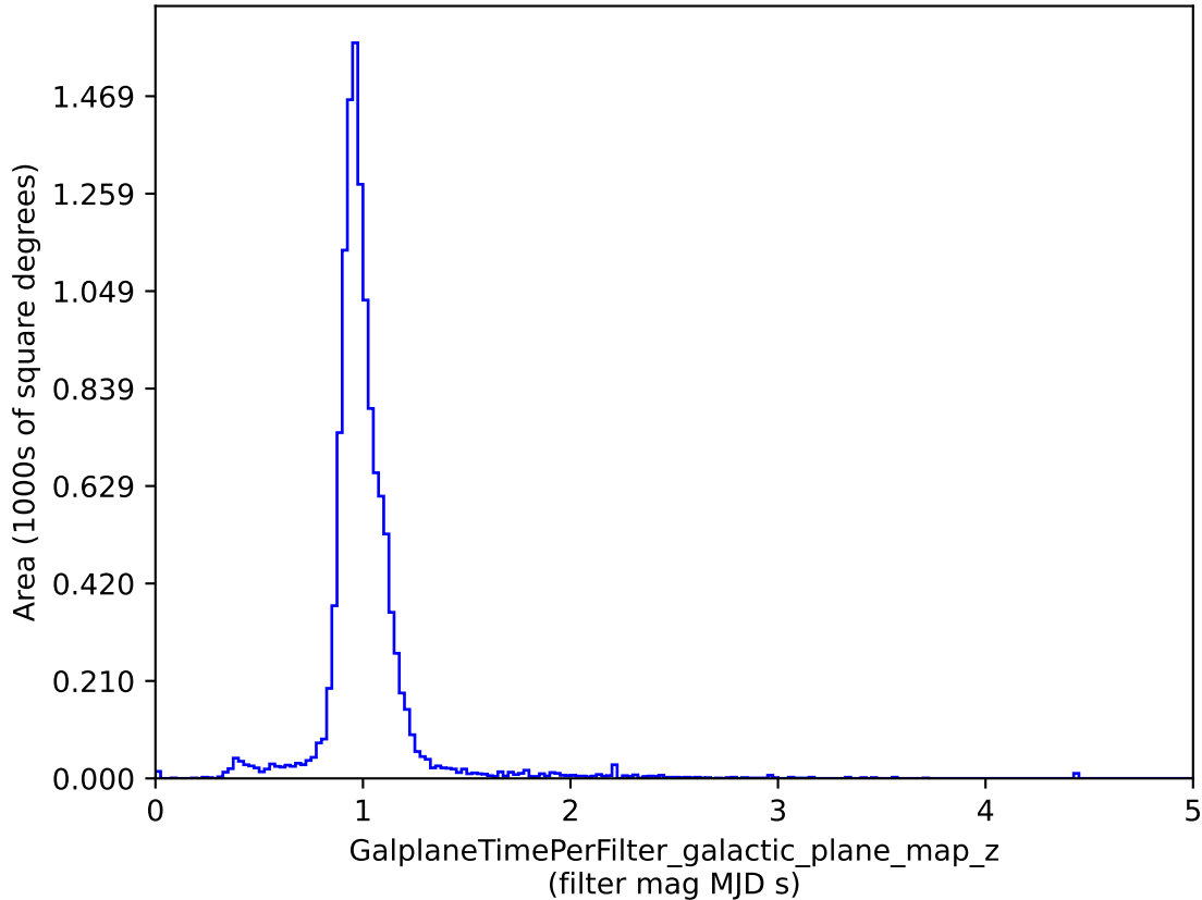
smc_lmc_v3.3_10yrs : GalplaneTimePerFilter_galactic_plane_map_z
