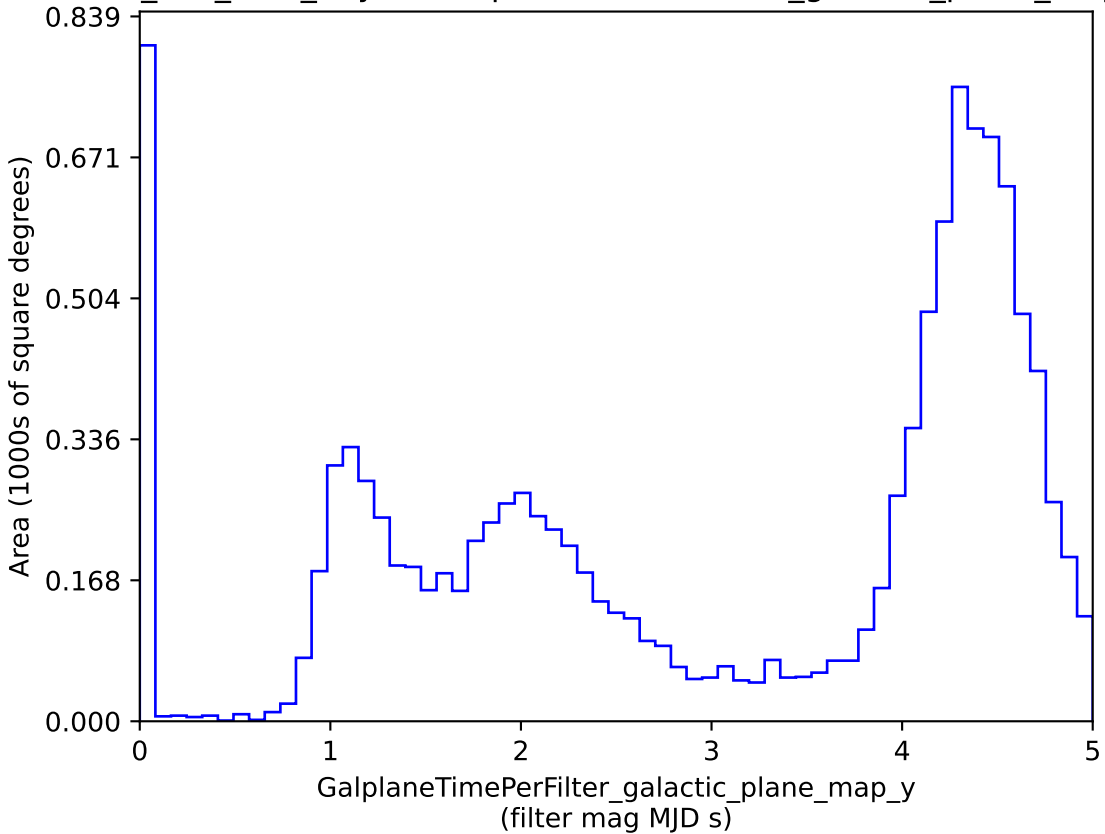
smc_lmc_v3.3_10yrs : GalplaneTimePerFilter_galactic_plane_map_y
