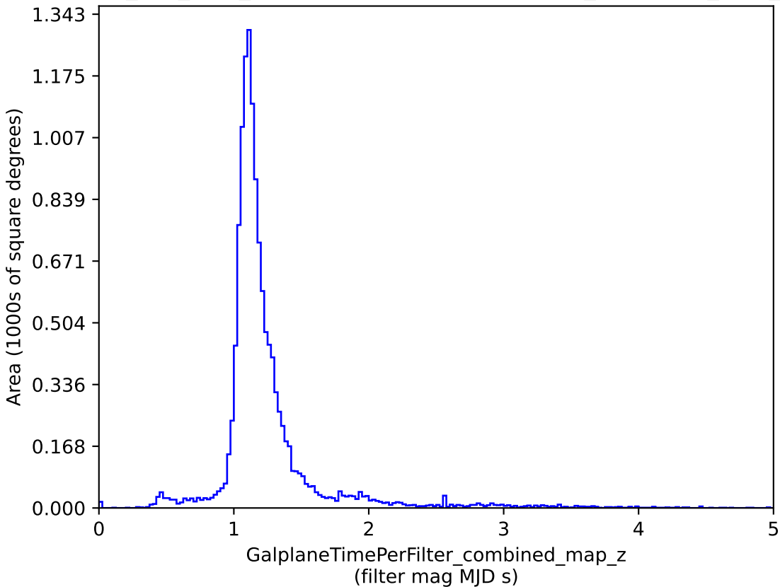
smc_lmc_v3.3_10yrs : GalplaneTimePerFilter_combined_map_z
