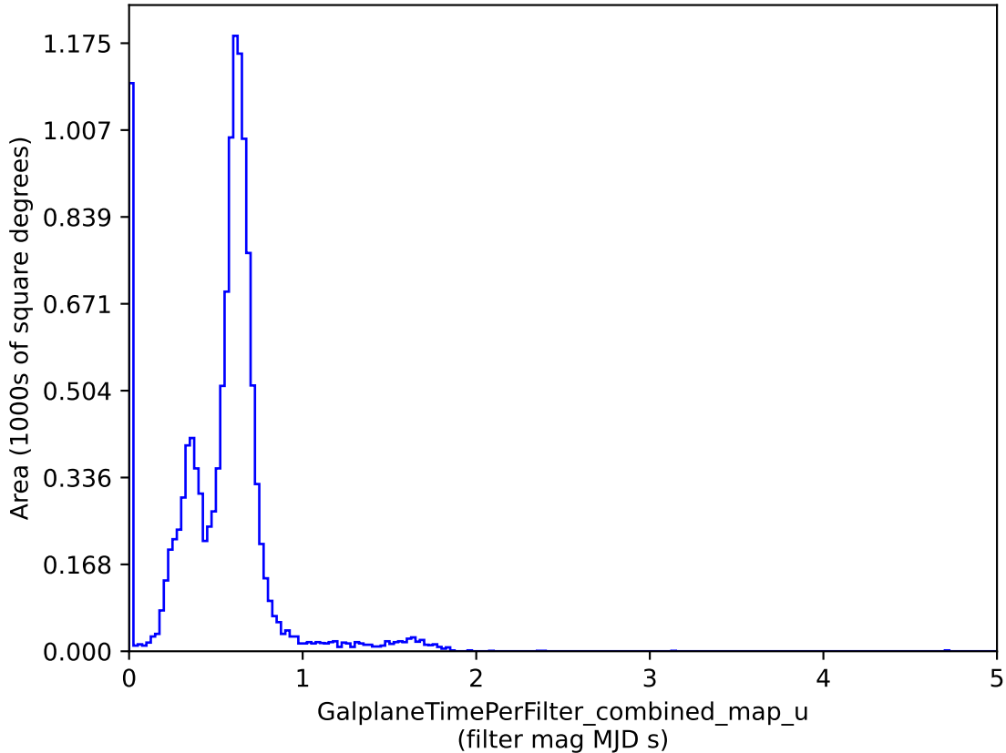
smc_lmc_v3.3_10yrs : GalplaneTimePerFilter_combined_map_u
