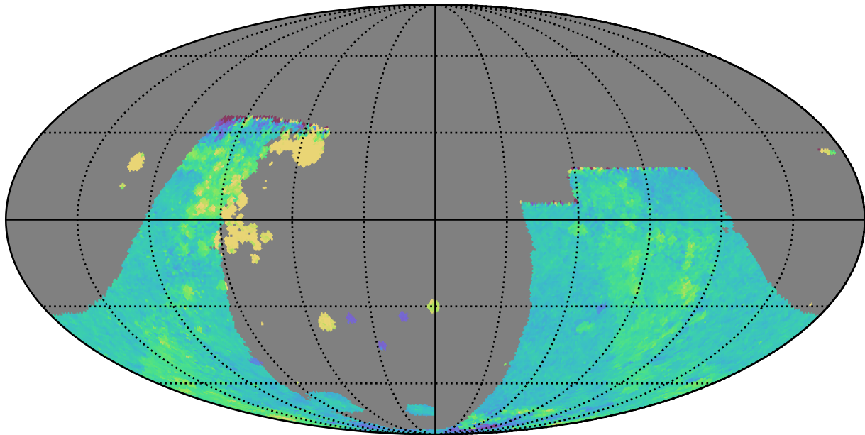
smc_lmc_v3.3_10yrs : GalplaneTimePerFilter_combined_map_r
