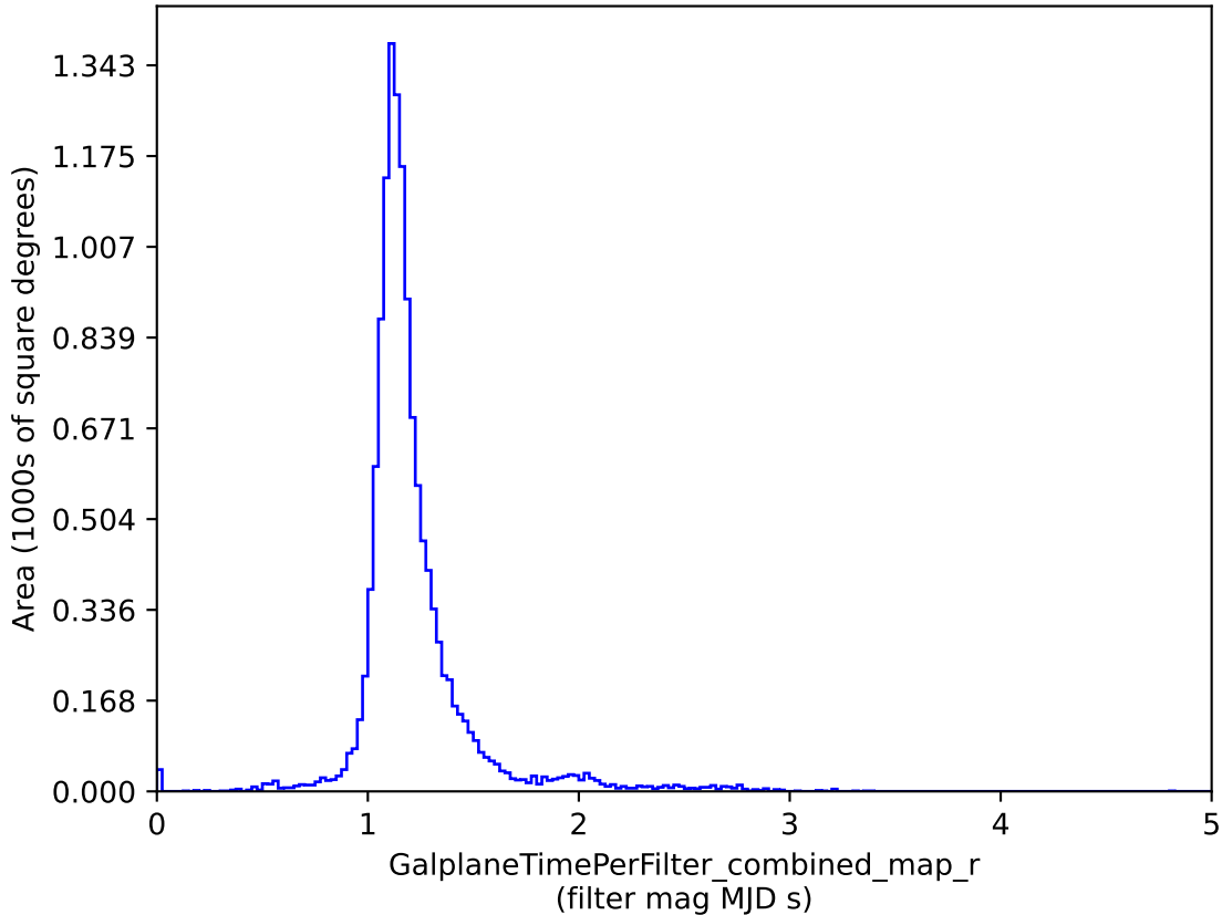
smc_lmc_v3.3_10yrs : GalplaneTimePerFilter_combined_map_r
