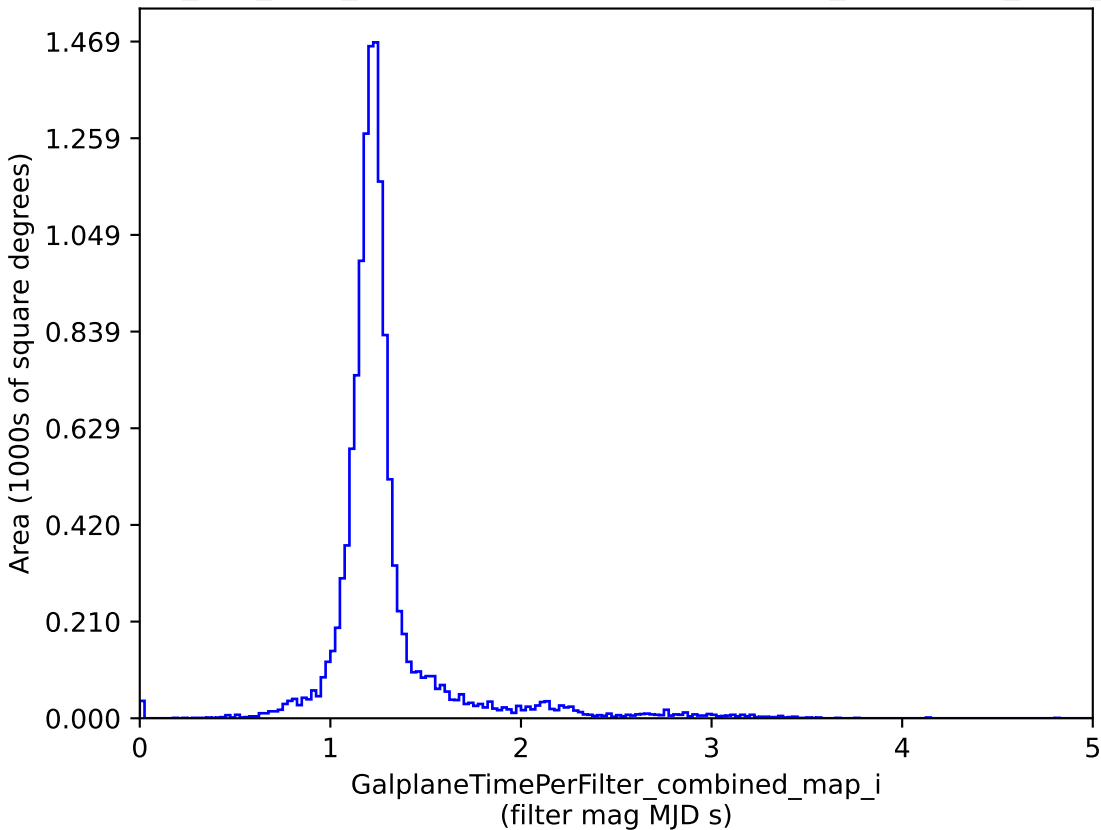
smc_lmc_v3.3_10yrs : GalplaneTimePerFilter_combined_map_i
