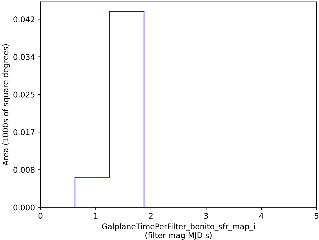
smc_lmc_v3.3_10yrs : GalplaneTimePerFilter_bonito_sfr_map_i
