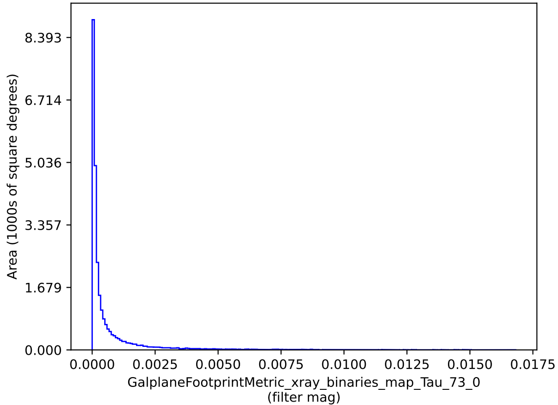
smc_lmc_v3.3_10yrs : GalplaneFootprintMetric_xray_binaries_map_Tau_73_0
