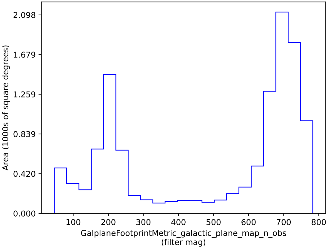
smc_Imc_v3.3_10yrs : GalplaneFootprintMetric_galactic_plane_map_n_obs
