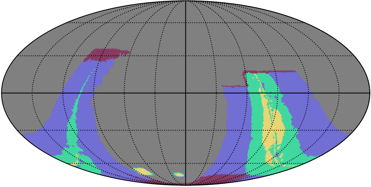
smc_lmc_v3.3_10yrs : GalplaneFootprintMetric_galactic_plane_map_Tau_46_5
