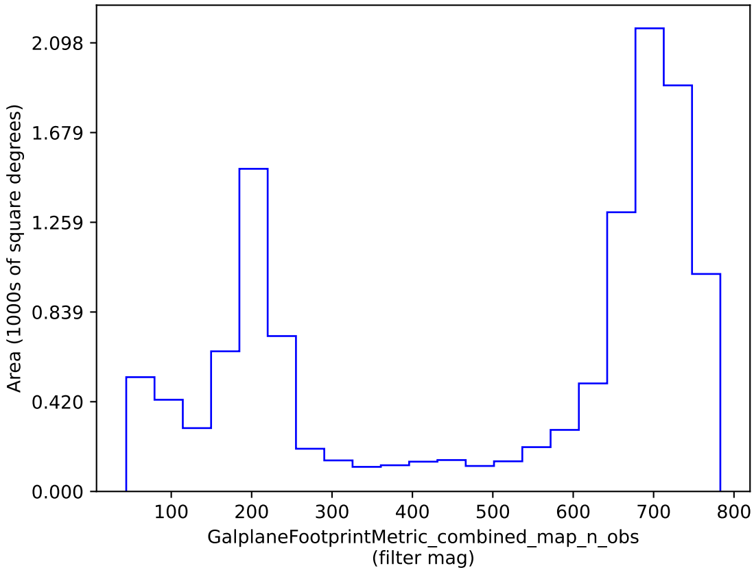
smc_lmc_v3.3_10yrs : GalplaneFootprintMetric_combined_map_n_obs
