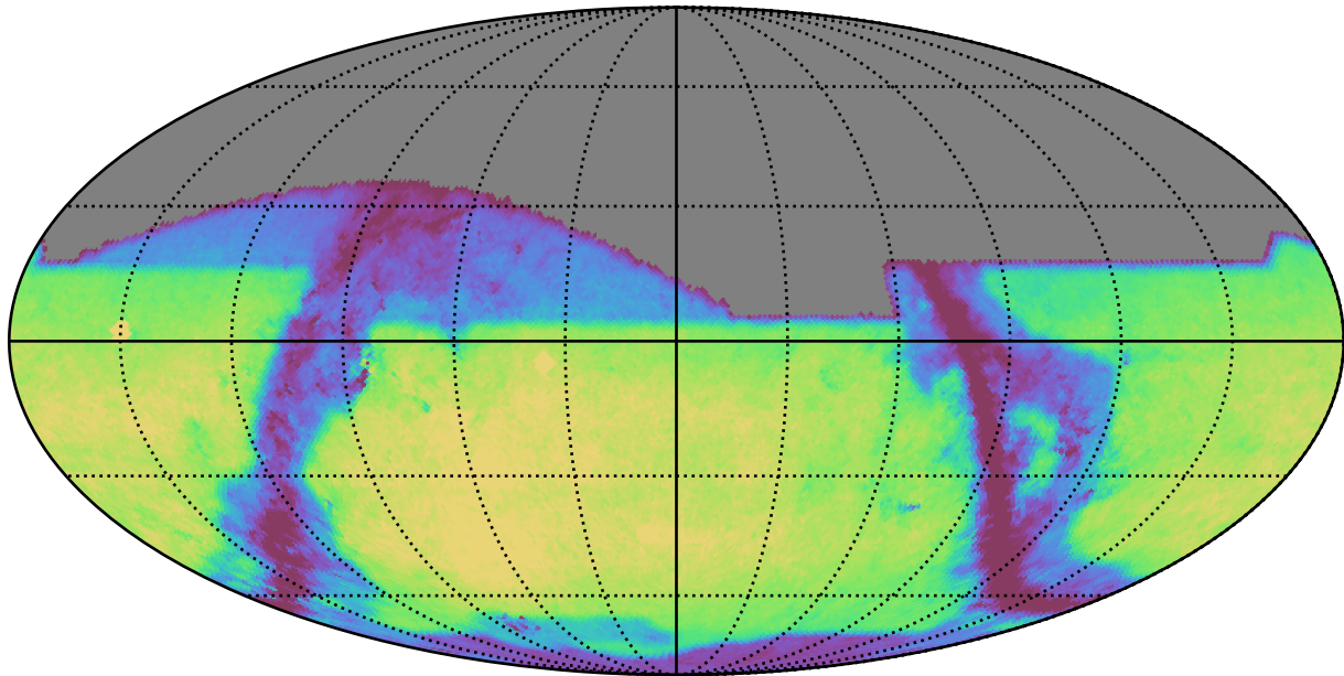
smc_lmc_v3.3_10yrs z: GalaxyCountsMetricExtended
