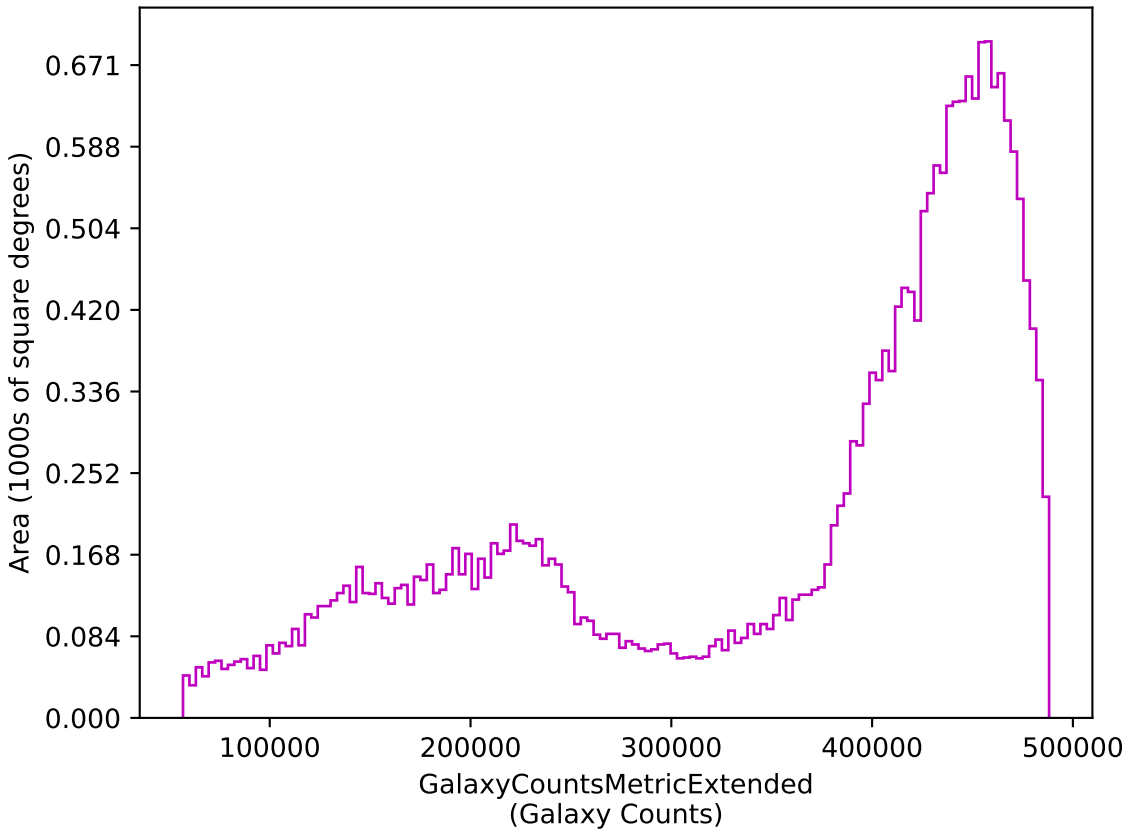
smc_lmc_v3.3_10yrs z: GalaxyCountsMetricExtended
