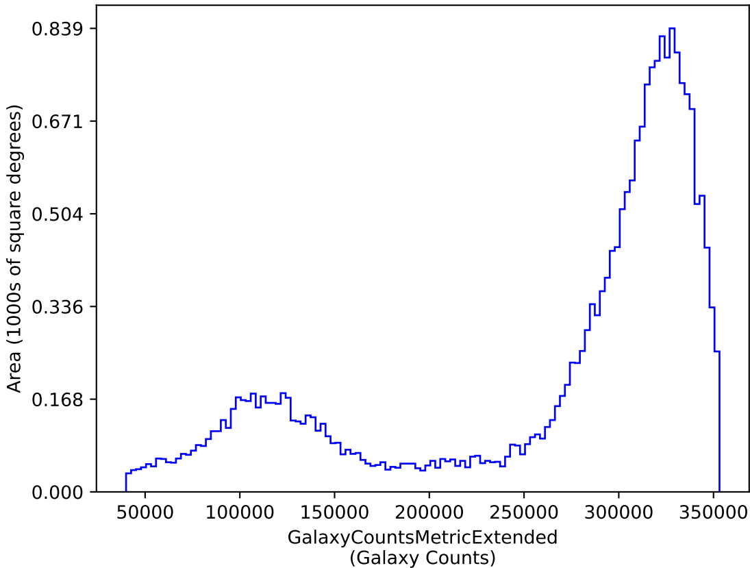
smc_lmc_v3.3_10yrs y: GalaxyCountsMetricExtended
