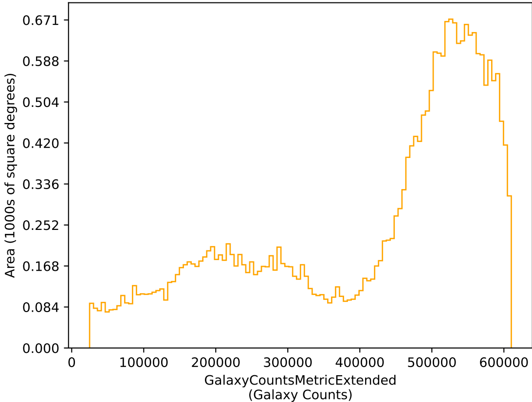
smc_lmc_v3.3_10yrs r: GalaxyCountsMetricExtended
