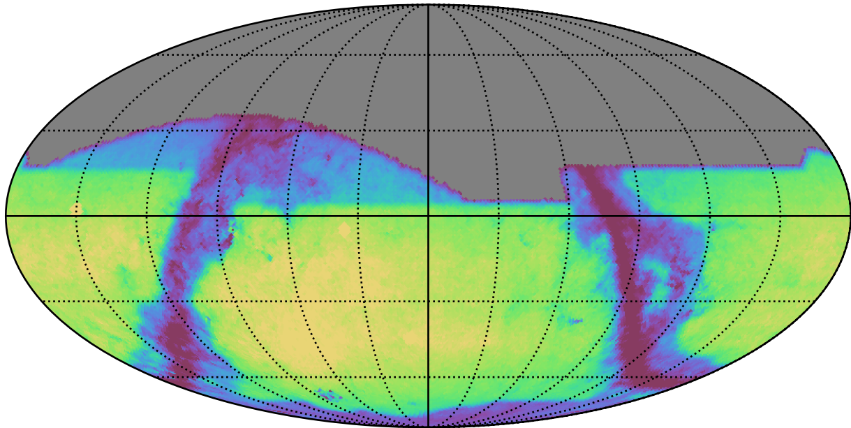
smc_lmc_v3.3_10yrs i: GalaxyCountsMetricExtended
