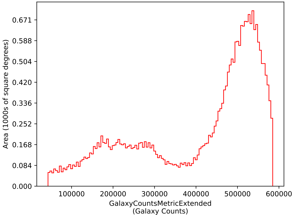
smc_lmc_v3.3_10yrs i: GalaxyCountsMetricExtended
