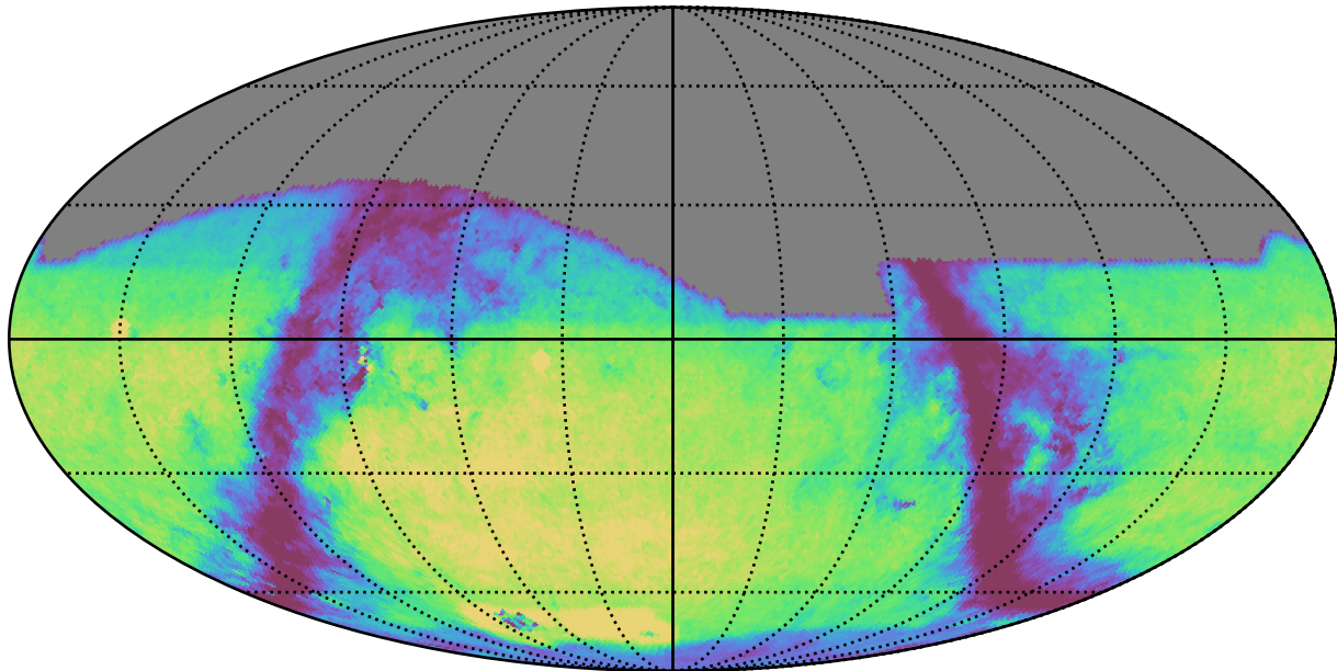
smc_lmc_v3.3_10yrs g: GalaxyCountsMetricExtended
