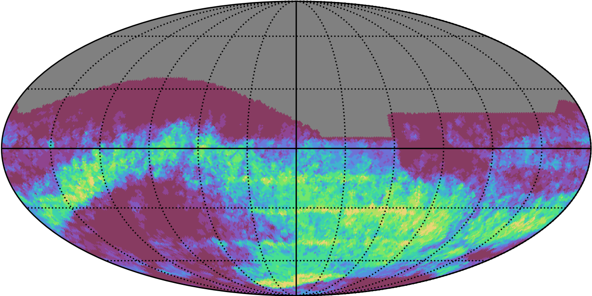
smc_lmc_v3.3_10yrs : GalPlaneSeasonGapsTimescales_xray_binaries_map_Tau_25_0
