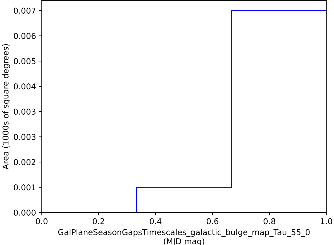
smc_lmc_v3.3_10yrs : GalPlaneSeasonGapsTimescales_galactic_bulge_map_Tau_55_0
