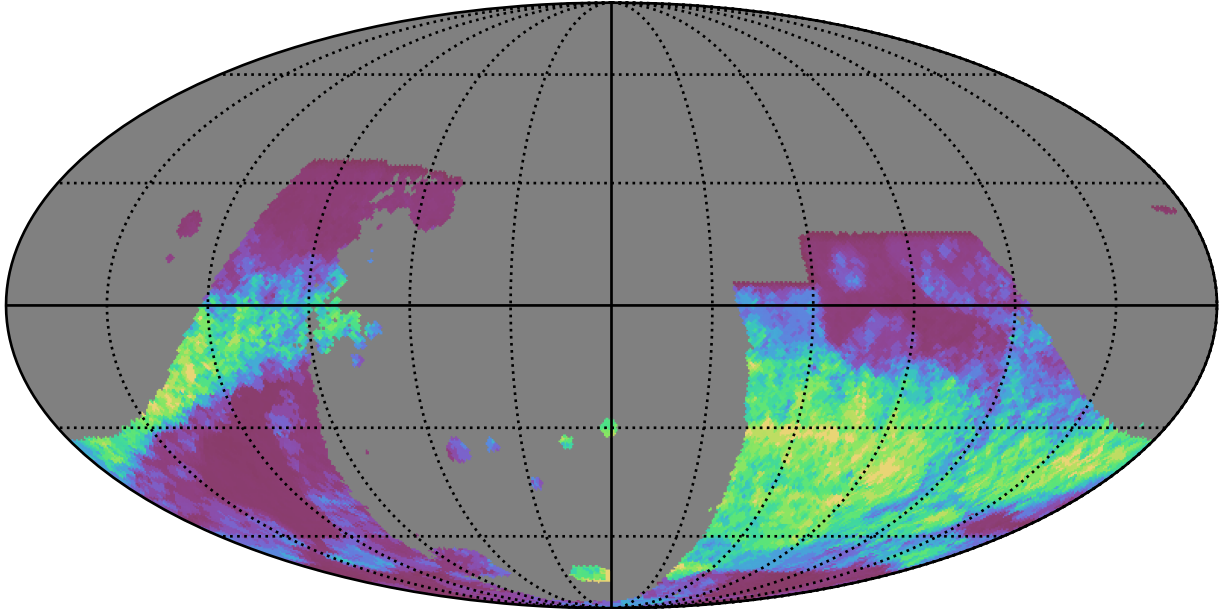
smc_lmc_v3.3_10yrs : GalPlaneSeasonGapsTimescales_combined_map_Tau_55_0
