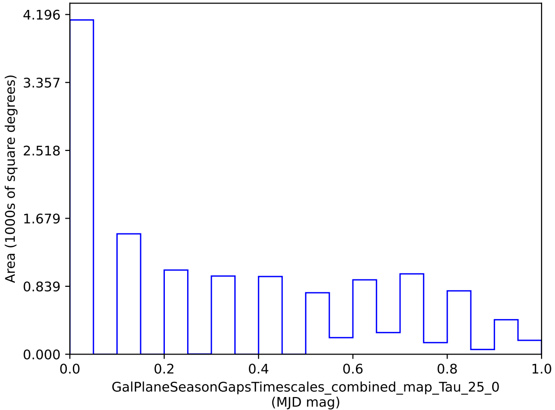
smc_Imc_v3.3_10yrs : GalPlaneSeasonGapsTimescales_combined_map_Tau_25_0
