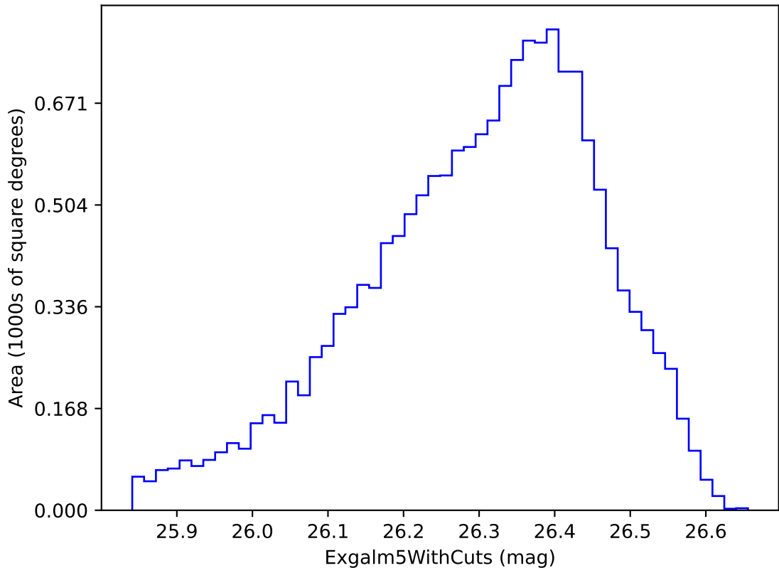
smc_lmc_v3.3_10yrs i band non-DD year 9: ExgalM5WithCuts
