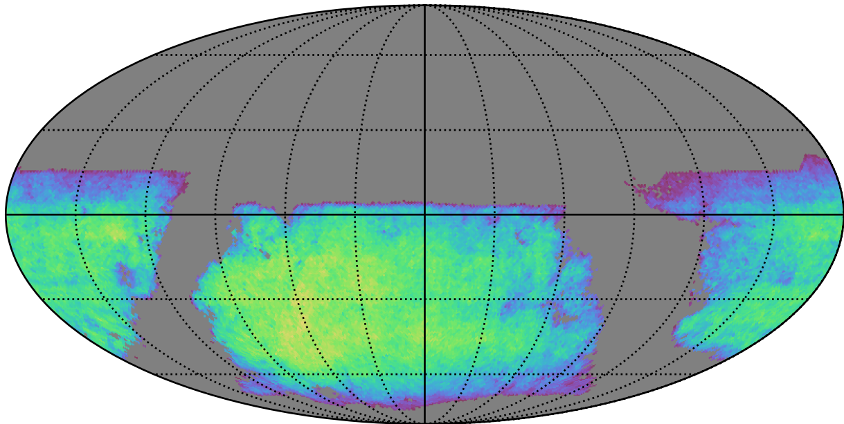
smc_lmc_v3.3_10yrs i band non-DD year 8: ExgalM5WithCuts
