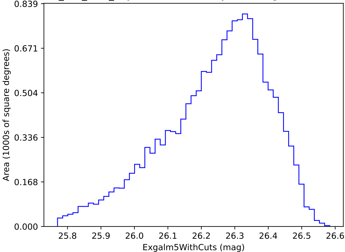
smc_lmc_v3.3_10yrs i band non-DD year 8: ExgalM5WithCuts
