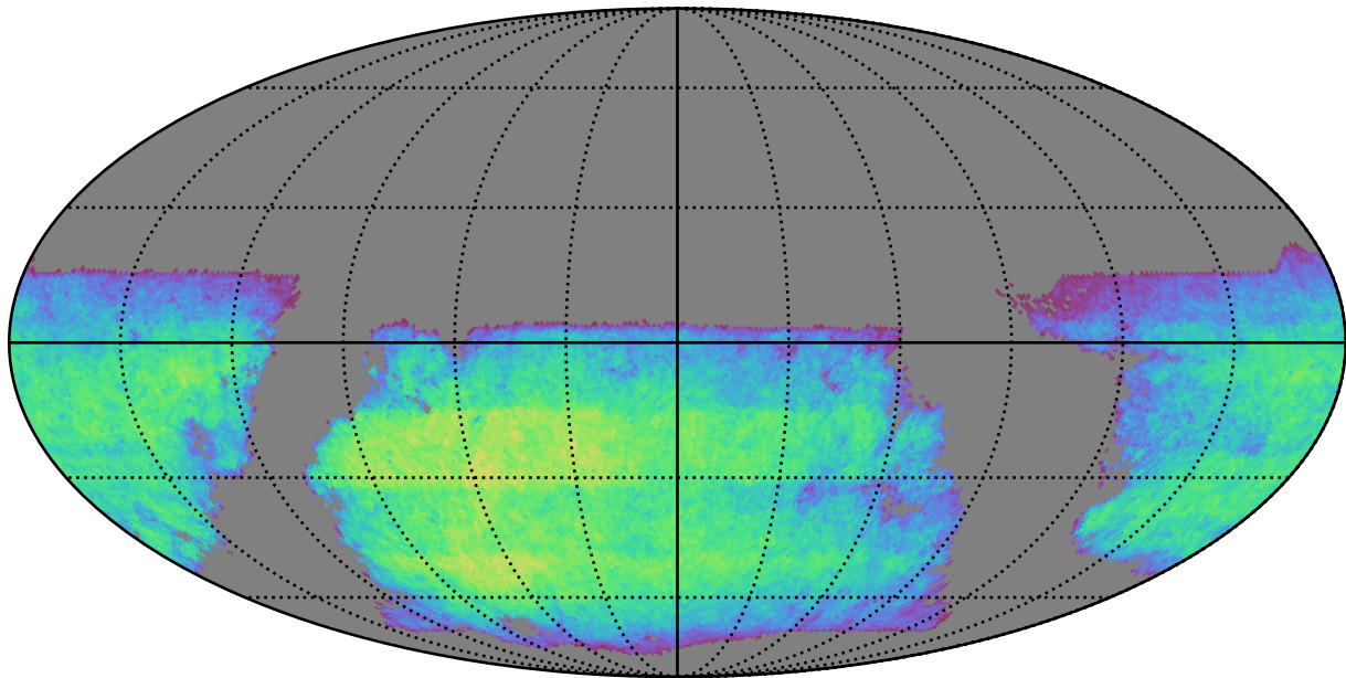
smc_lmc_v3.3_10yrs i band non-DD year 7: ExgalM5WithCuts
