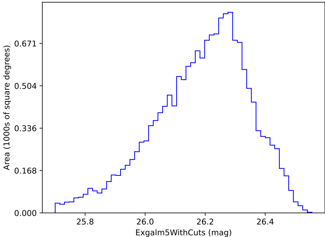
smc_lmc_v3.3_10yrs i band non-DD year 7: ExgalM5WithCuts
