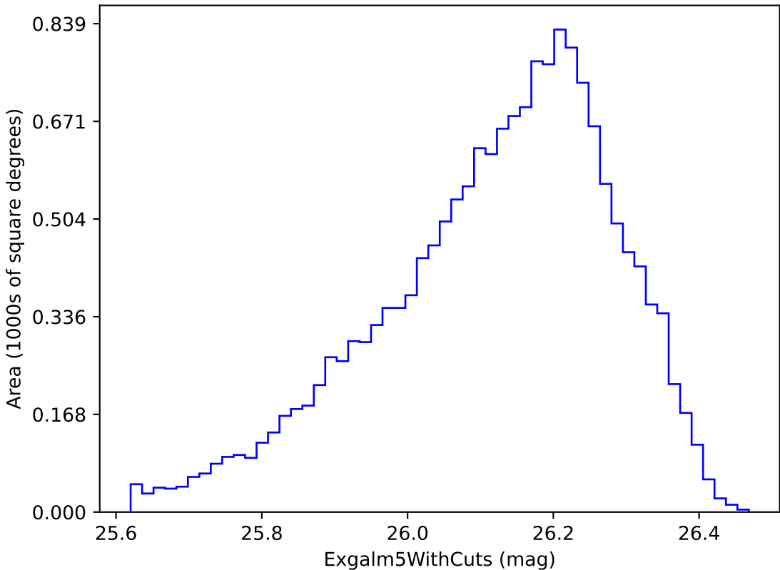
smc_lmc_v3.3_10yrs i band non-DD year 6: ExgalM5WithCuts
