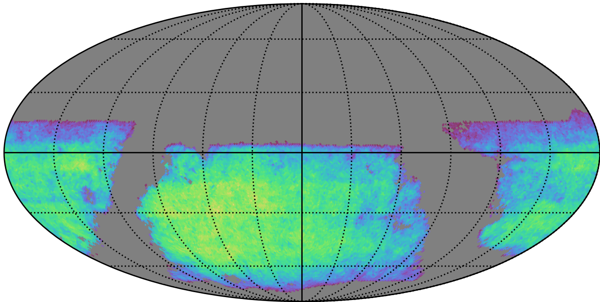
smc_lmc_v3.3_10yrs i band non-DD year 4: ExgalM5WithCuts
