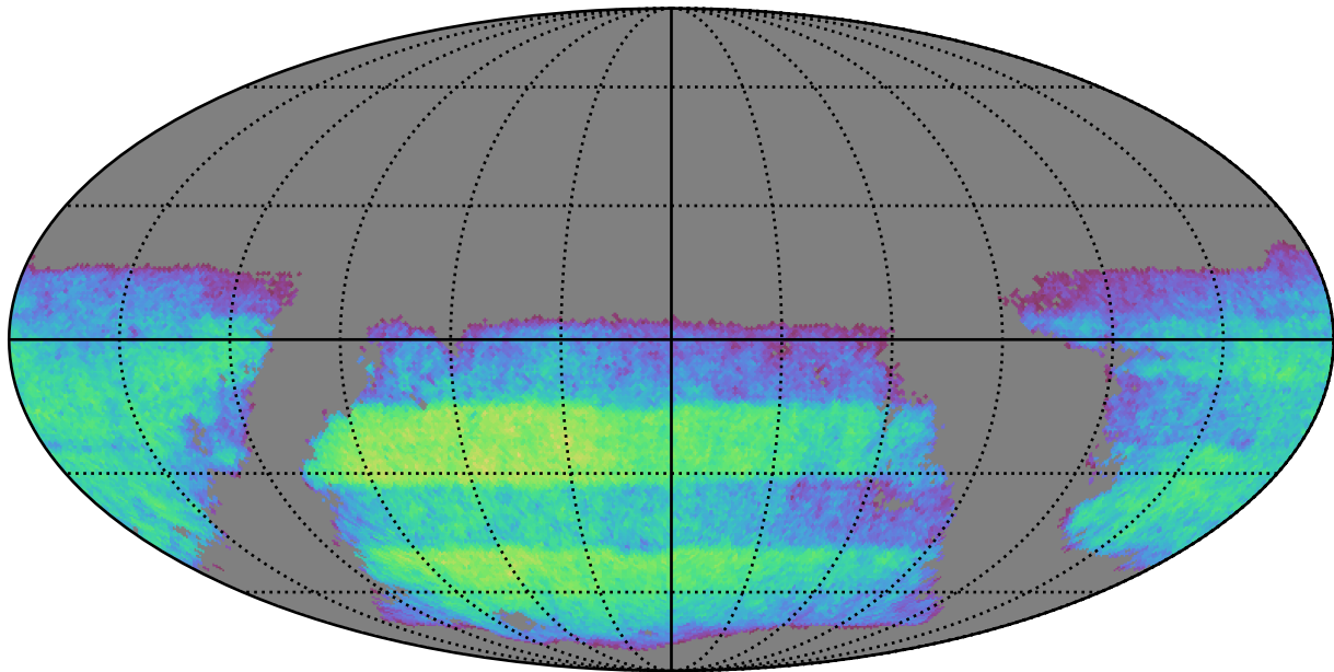
smc_lmc_v3.3_10yrs i band non-DD year 3: ExgalM5WithCuts
